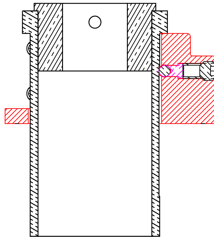
SECTION C-C
